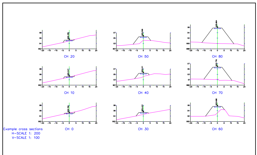
Cross sections produced automatically
