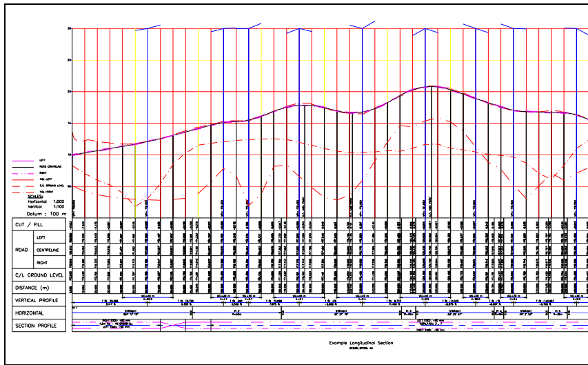
Typical longitudinal section produced automatically
